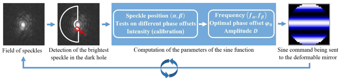
Fig.3. SN algorithm principle. The coronagraphic PSF is used as an input. In the desired dark hole, the brightest speckle is selected. Thanks to its position, the frequency of the optimal correction sine function is computed. The amplitude of the correction function is obtained thanks to a calibration step and the intensity of the speckle. The optimal phase offset is deduced from test commands that are sent to the DM before selection of the most efficient one. After correction of the speckle, the second brightest speckle is selected in the dark hole, and the algorithm is applied again.
